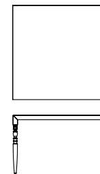
NA/8 cm. 120x120x74h. inch 47,25x47,25x29,25h.
